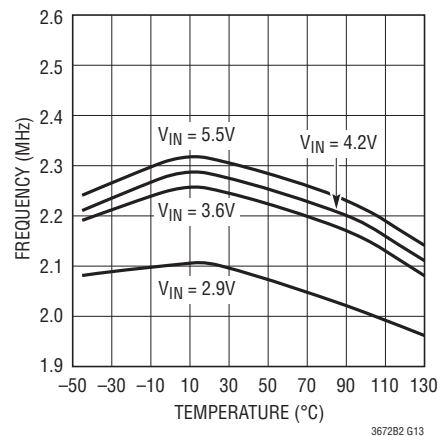
Buck Oscillator Frequency vs Temperature
